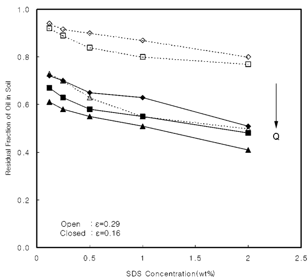
Fig. 3. Residual oil fraction in soil after exhaustive washing at different SDS concentrations. ♦: V_s = 0.757 cm/min; ■: V_s = 1.742 cm/min; ▲: V_s = 2.575 cm/min.
