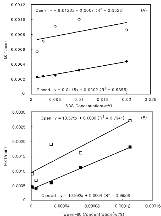
Fig. 12. Dependence of the model parameter, k_0 on the surfactant concentrations of (a) SDS and (b) Tween-80. Open symbol: \varepsilon = 0.16 ; closed one: \varepsilon = 0.29 .
