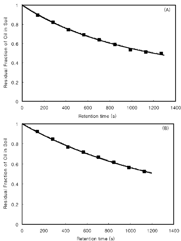
Fig. 13. Two examples of model calculation compared to the corresponding experimental data for (a) an SDS solution ( C=2.0 wt%, \epsilon=0.29 and V_s=2.575 cm/min) and (b) another SDS solution ( C=0.5 wt%, \epsilon=0.16 and V_s=2.575 cm/min). Solid lines denote model calculation results.
