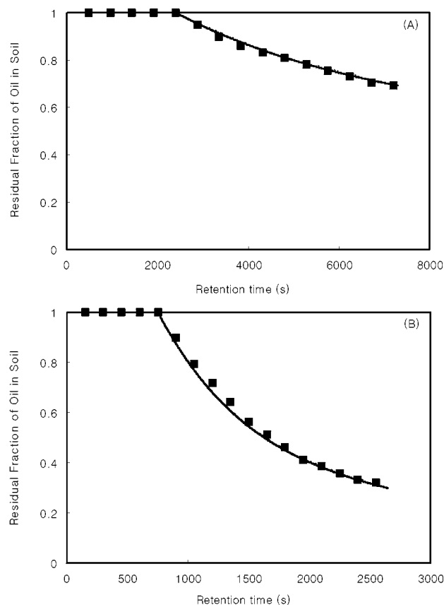
Fig. 14. Two examples of model calculation compared to the corresponding experimental data for (a) a Tween-80 solution ( S=0.0065 wt%, \epsilon=0.29 and V_s=0.757 cm/min) and (b) another Tween-80 solution ( S=0.013 wt%, \epsilon=0.29 and V_s=2.575 cm/min). Solid lines denote model calculation results.
