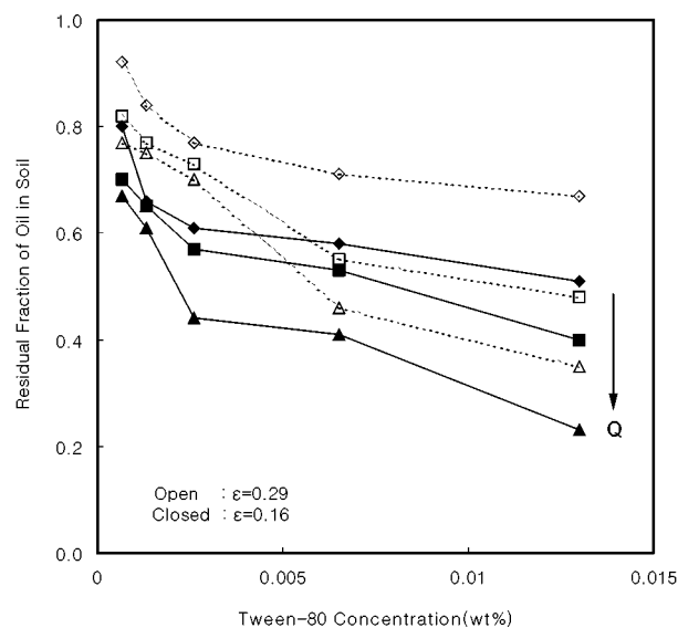
Fig. 4. Residual oil fraction in soil after exhaustive washing at different Tween-80 concentrations. ♦: V_s = 0.757 cm/min; ■: V_s = 1.742 cm/min; ▲: V_s = 2.575 cm/min.
